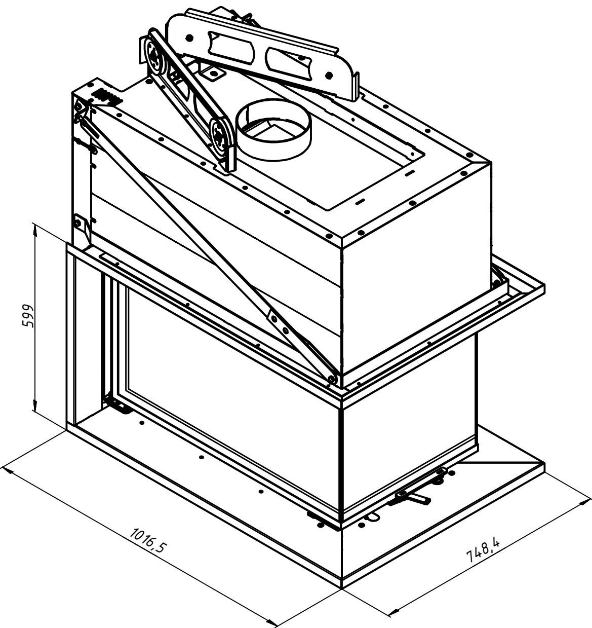
Mounting frame 1.5mm 1x90
